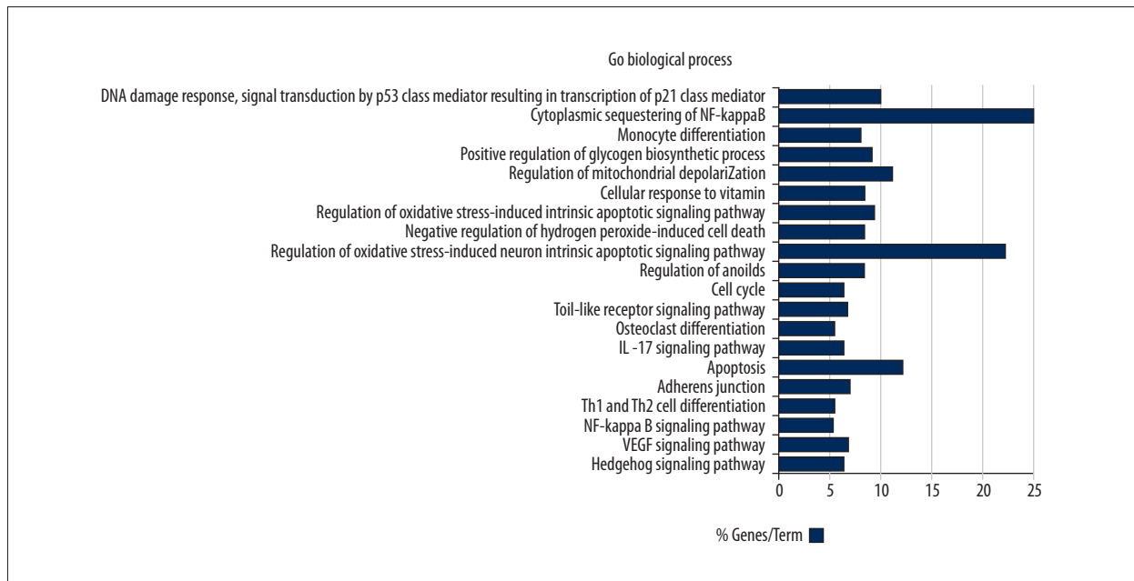
Figure 4. GO biological process analysis. Go – Gene Ontology.
