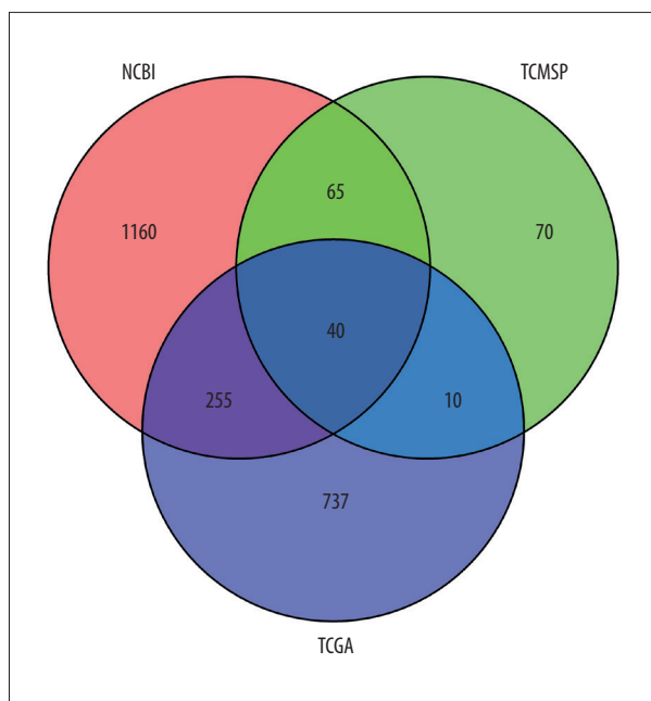
Figure 1. Screening of potential anti-NSCLC targets of Artemisia annua. NSCLC – non-small cell lung cancer.
