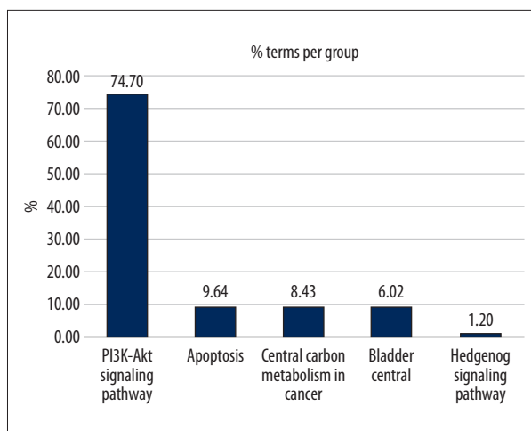
Figure 5. Enrichment analysis of KEGG signaling pathway. KEGG – Kyoto Encyclopedia of Genes and Genomes.
