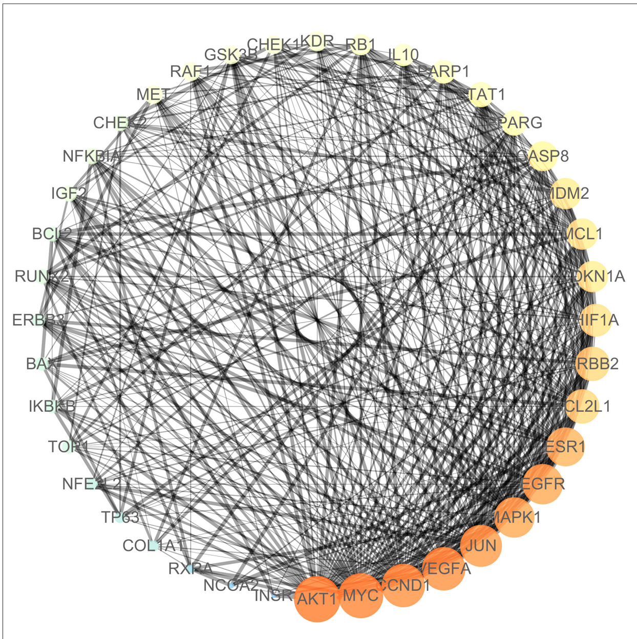
Figure 2. PPI network of Artemisia annua potential target for NSCLC treatment. PPI – protein–protein interactions; NSCLC – non-small cell lung cancer.
