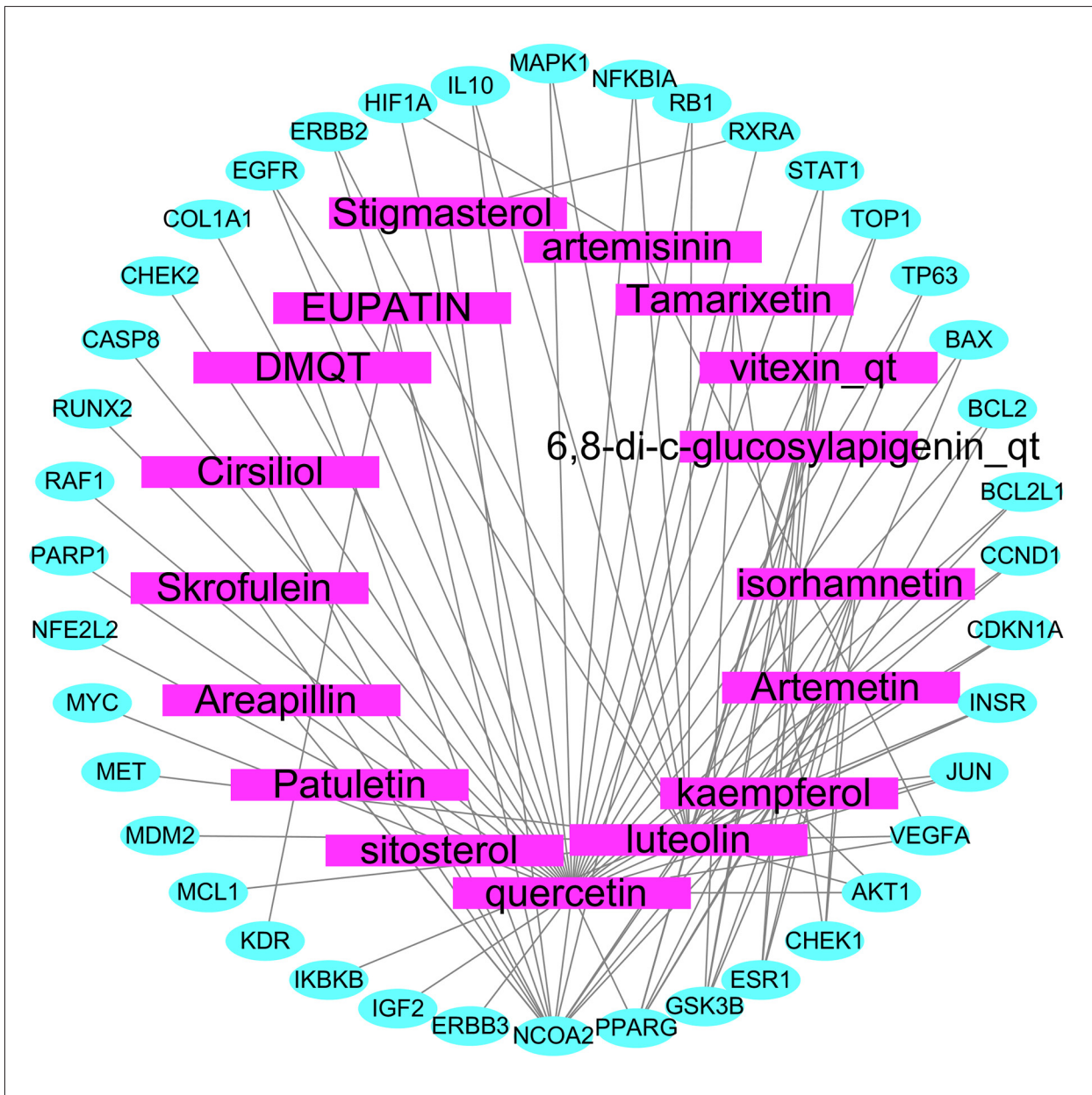
Figure 3. Network map of active ingredients and targets of Artemisia annua in the treatment of NSCLC. NSCLC – non-small cell lung cancer.
